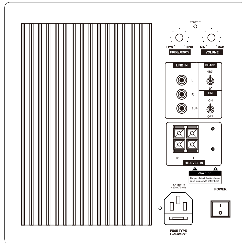
Fig. 1 Schematic Diagram of SUB-10-N Amplifier
